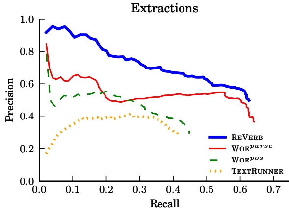
Figure 4: REVERB achieves significantly higher precision than state-of-the-art Open IE systems, and comparable recall to WOE^{parse} .
